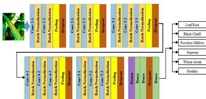
Figure 3: Flow diagram of proposed wheat leaf Convolution (WLC) model
