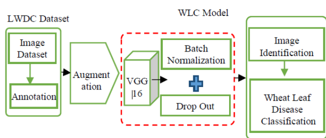
Figure 2: Overview of the Wheat Leaf Convolution (WLC) model
