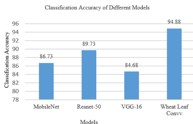
Figure 4: Classification of accuracies of all the selected models
