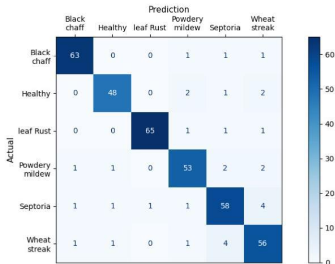
Figure 5: Confusion matrix for wheat leaf classification using WLC model
